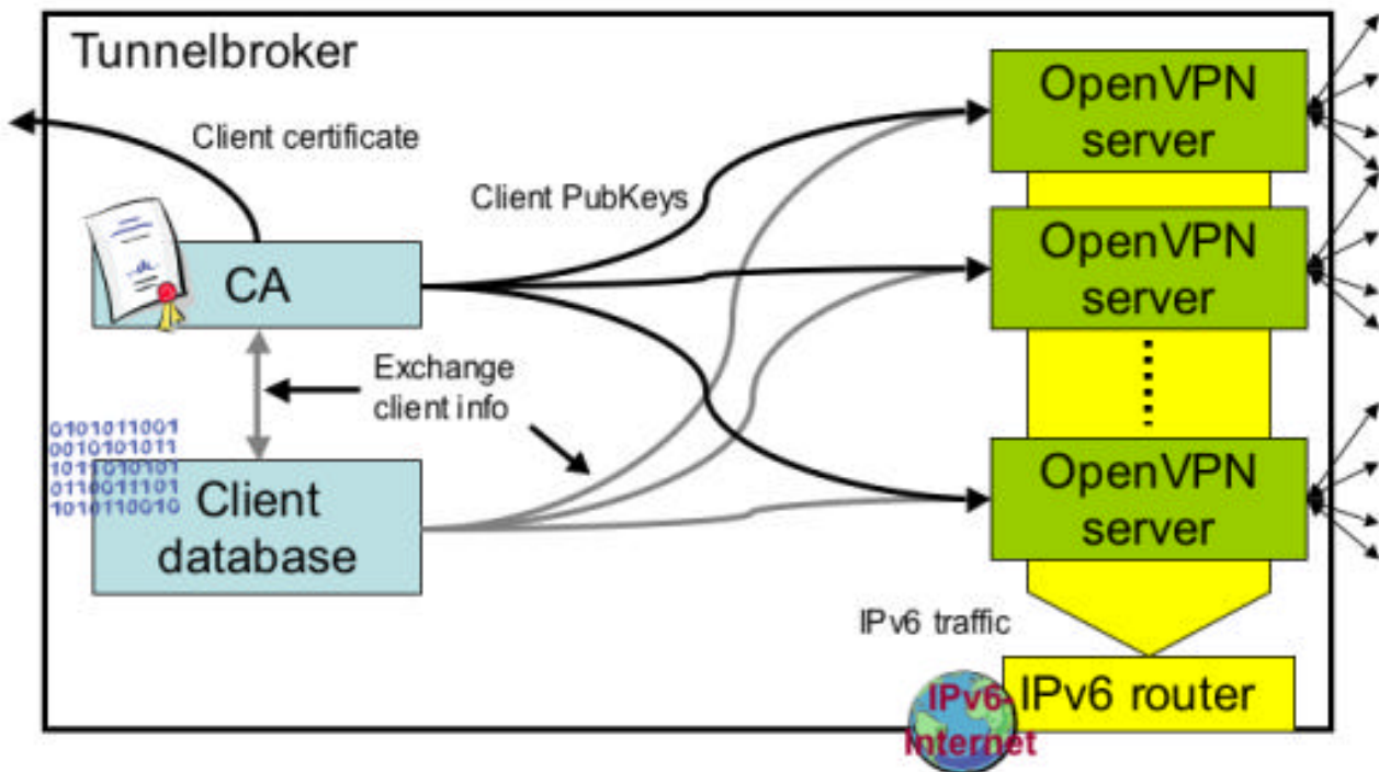
Figure 6-1 Interaction of tunnel broker components
