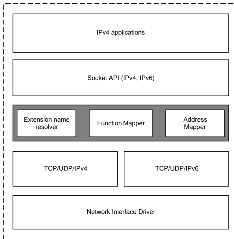
Figure 3-5: The BIA Protocol Stack
